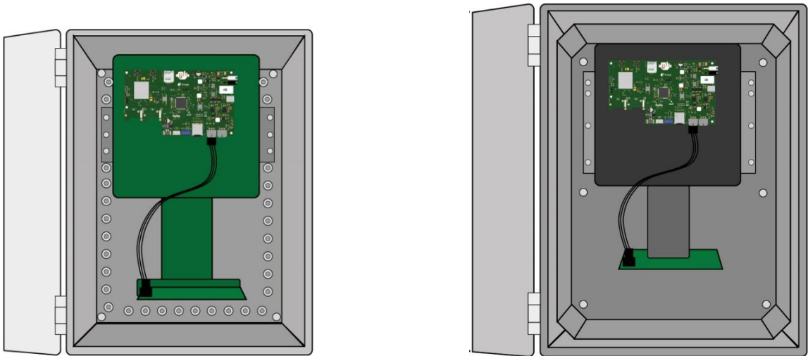
Figure 7: Detector F3 (left) and Detector F5 (right)
