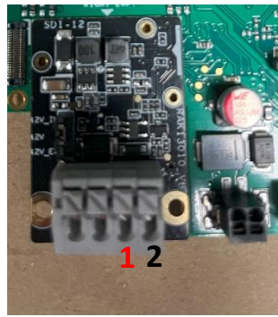
Figure 30: SDI12 module to data logger connections: 1 - DATA, 2 - GND
