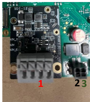
Figure 29: SDI12 module to data logger connections: 1 - DATA, 2 - GND, 3 – 12V
