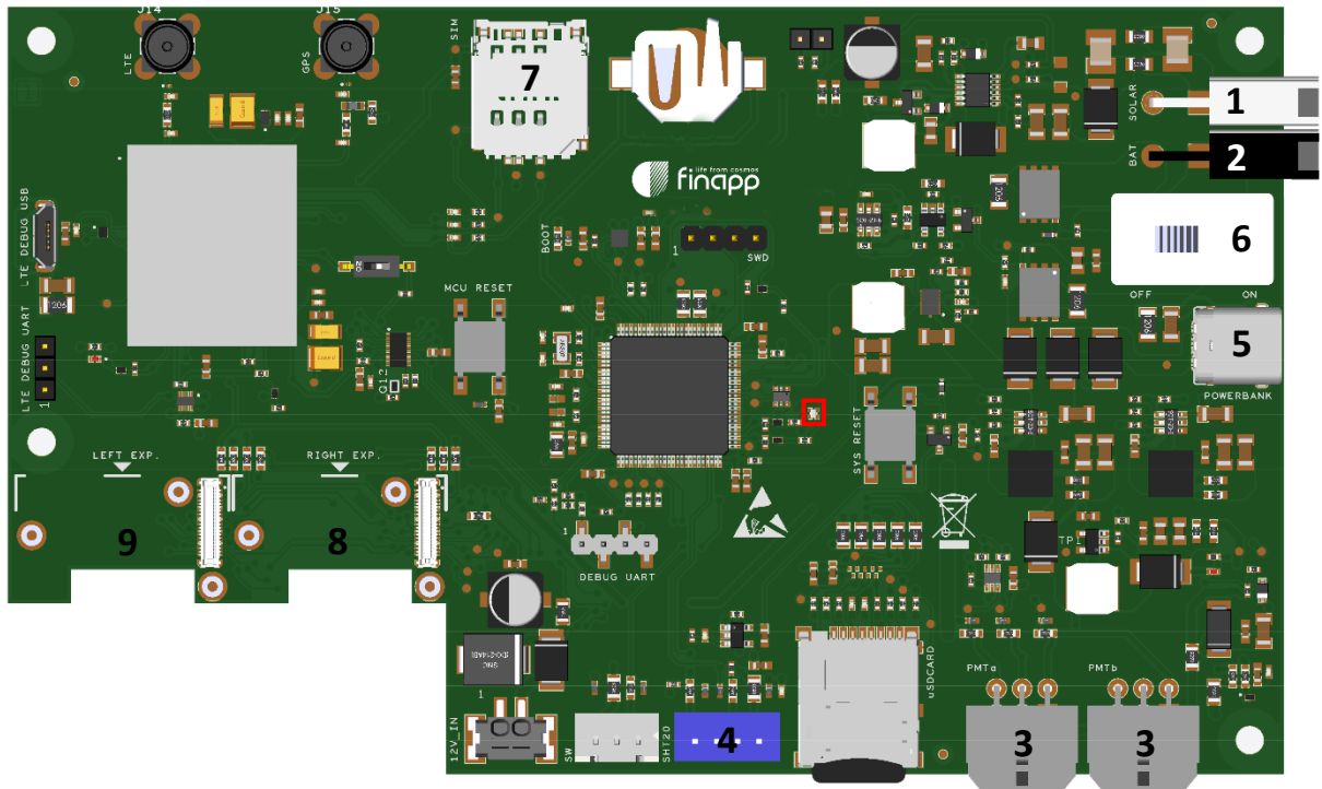
Figure 3: Details of the Master board. 1 - MOLEX of solar panel, 2 - MOLEX of the battery, 3 - PMT connectors, 4 - SHT20, red square – LED for debug, 5 - USB-C for indoor use, 6 – Switch, 7 – SIM card slot, 8 – Expansion slot 1 for RAK external modules, 9 – Expansion slot 2 for RAK external modules
