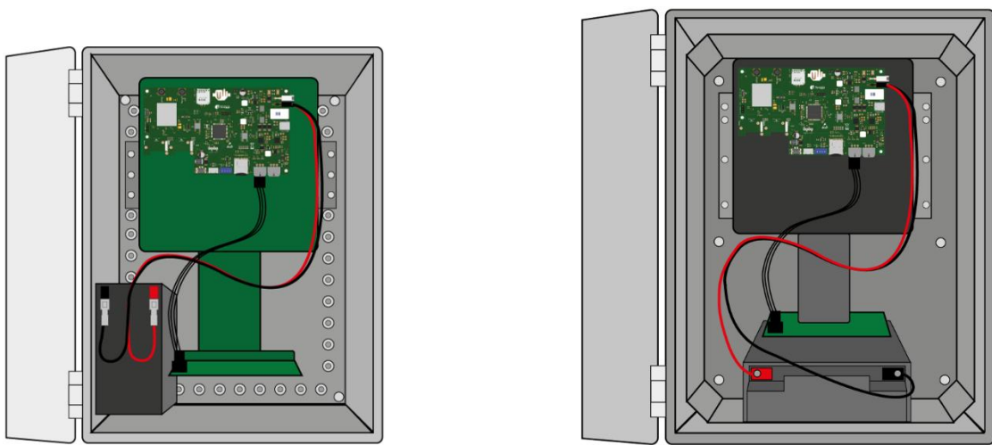
Figure 17: Finapp with 9Ah battery (left) and Finapp Plus with 18Ah battery (right)
